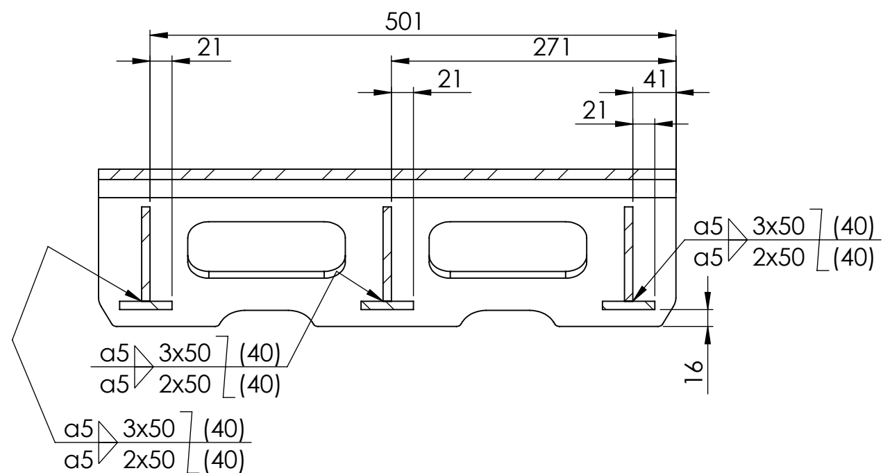
SECTION C-C
